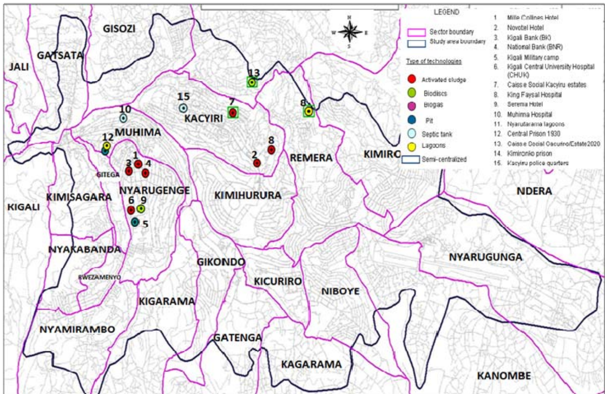
Fig. (2). Map showing the location of existing wastewater treatment plants and respective technologies applied in the CoK (Electrogaz, 2007).
